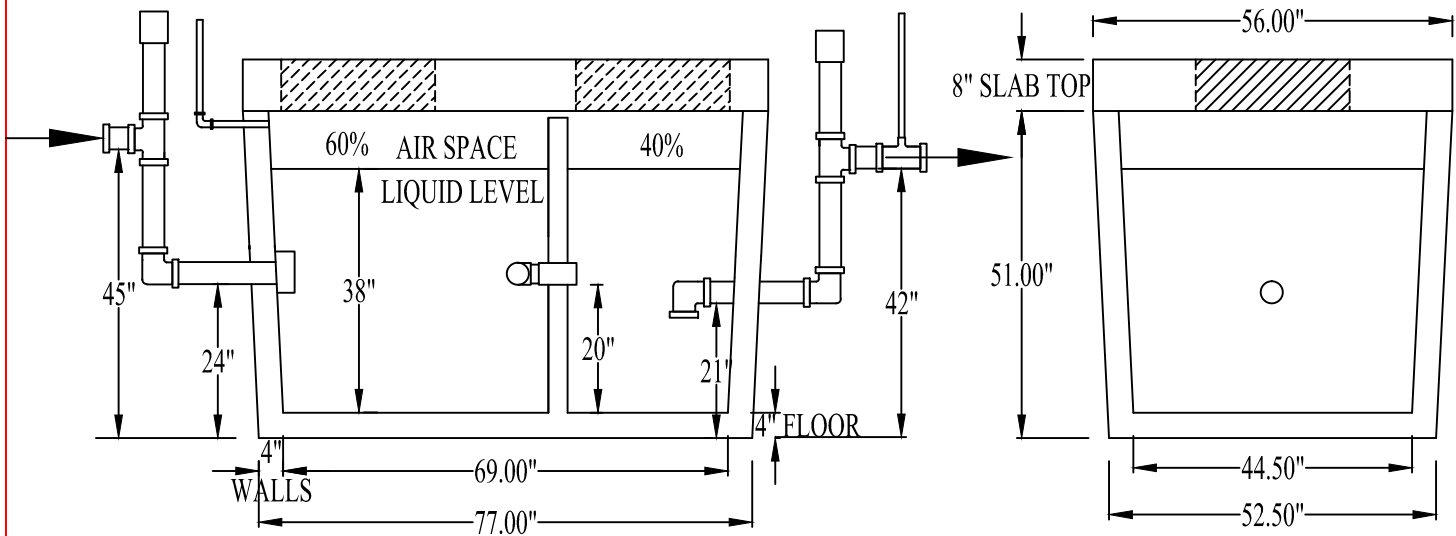
SIDE WALL DETAIL
