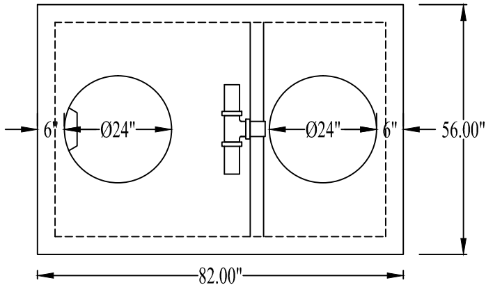
SLAB TOP DETAIL
